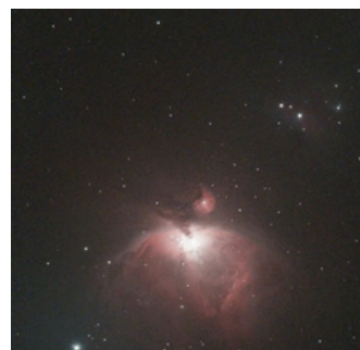
SEESTAR 30 DIGITAL TELESCOPE PHOTO TAKEN AT THE STANSBURY PARK OBSERVATORY COMPLEX OF THE M42 IS THE ORION NEBULA
